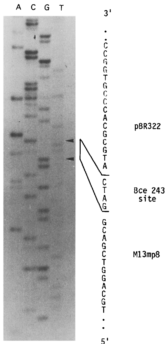
Fig.3. Sequence determination around the Bam HI cloning site of a M13mp8-derived recombinant phage containing a pBR322 fragment generated with Bce 243. Sequencing was done according to the dideoxy chain termination method [6] using an 8% denaturing polyacrylamide gel.
